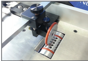
Bottom Vacuum Feed with Register Guide
